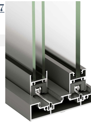
Section No.: AS-3104 Weight (Kg/12'): 5.110
