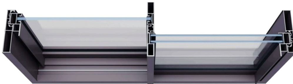
Section No.: AS-3110 Weight (Kg/12'): 4.980
